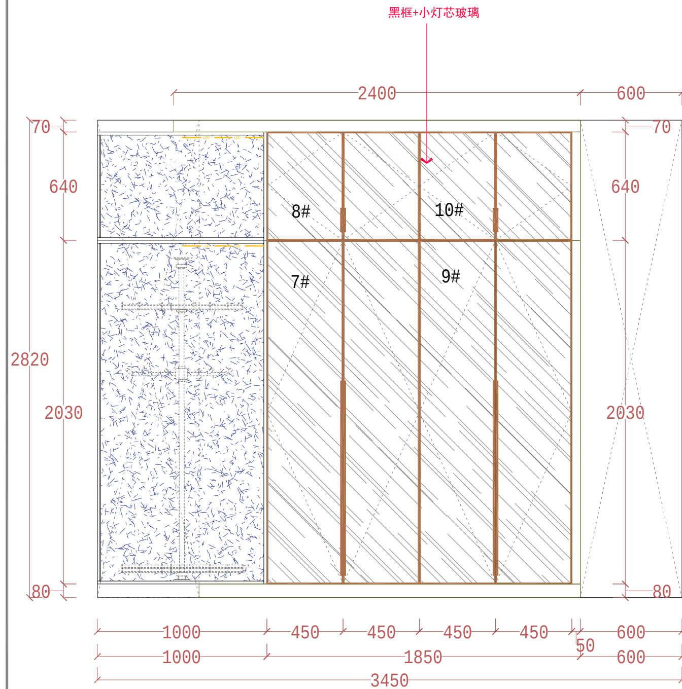
OUTSIDE VIEW B
