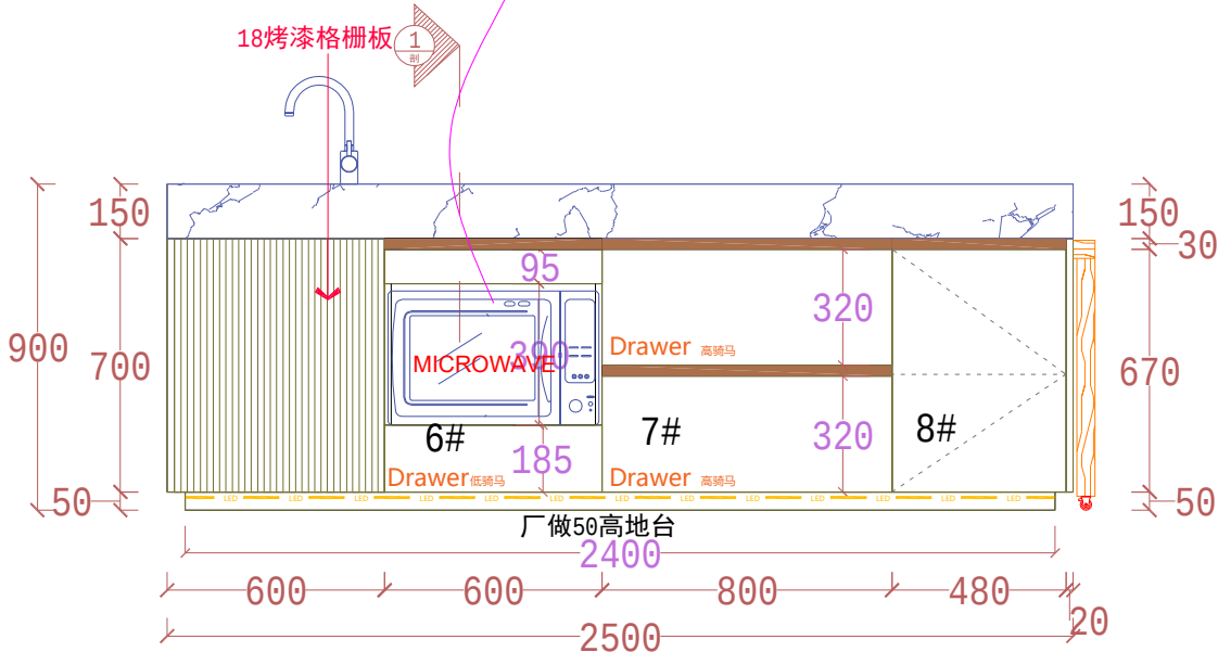
ELEVATION D
