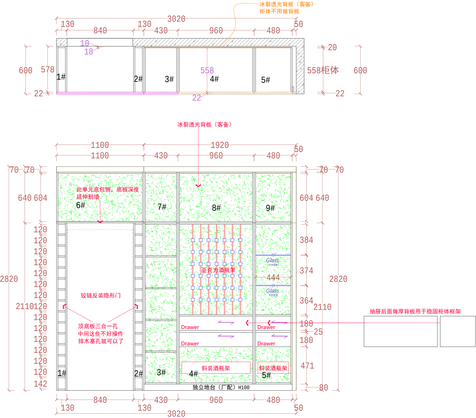
INNER VIEW
