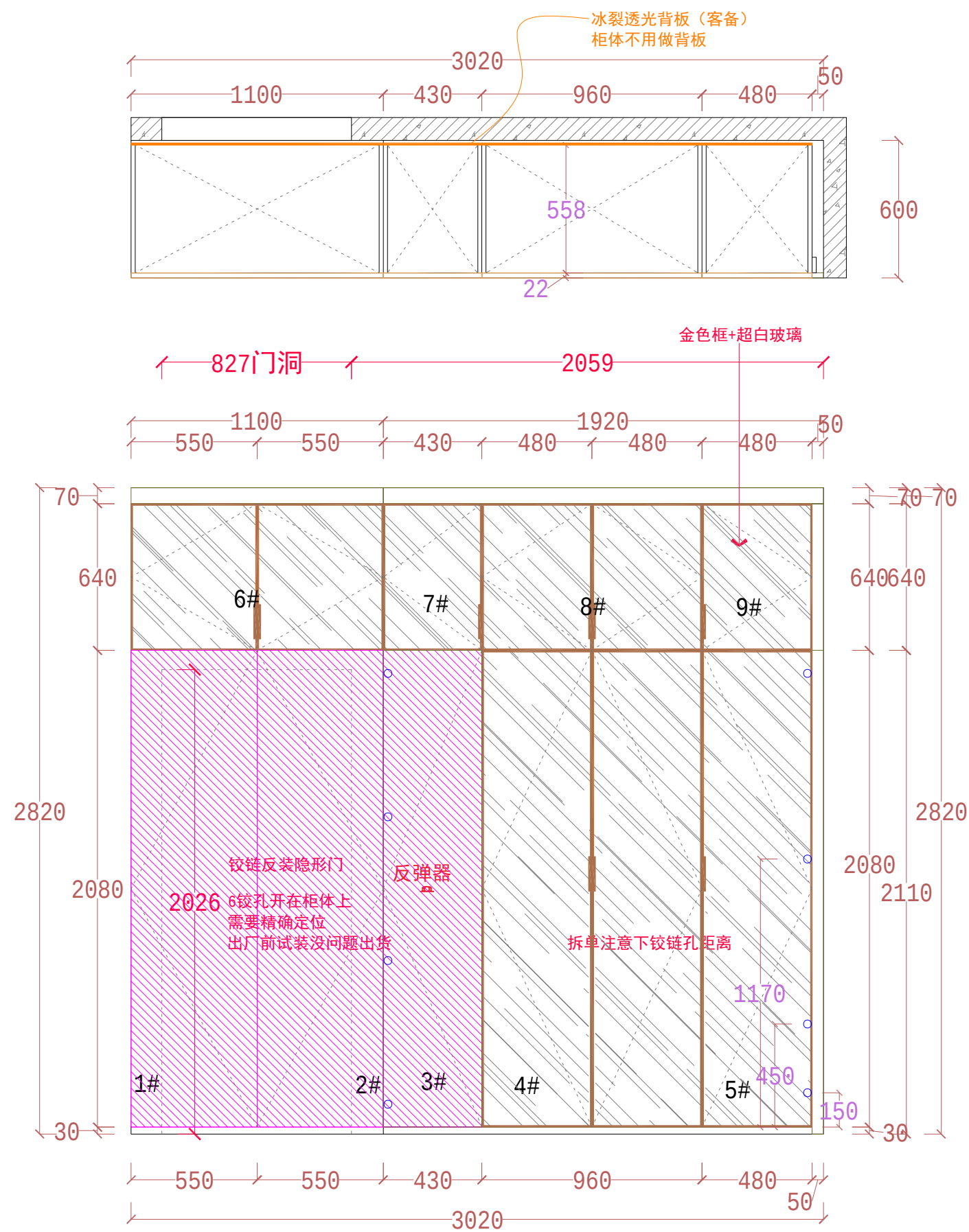
OUTSIDE VIEW
