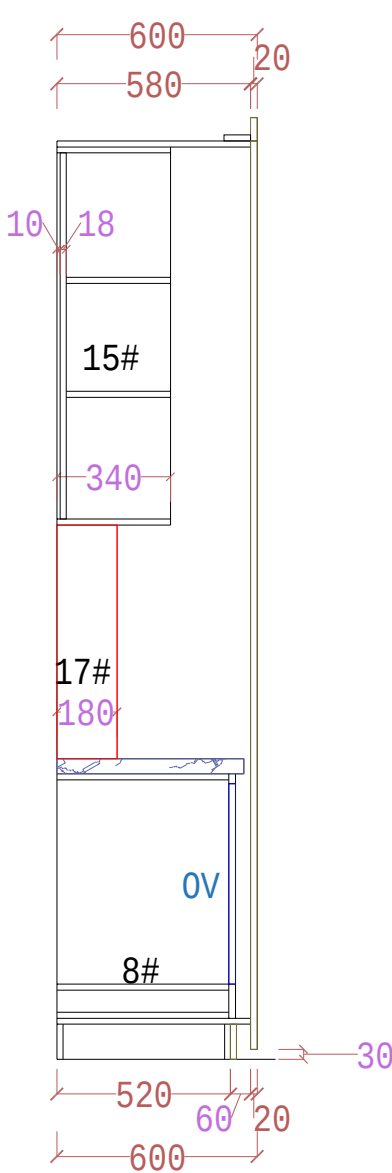
SECTION VIEW 1
