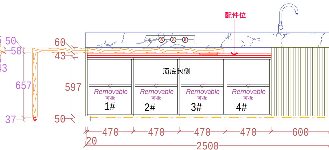
INNER VIEW B
