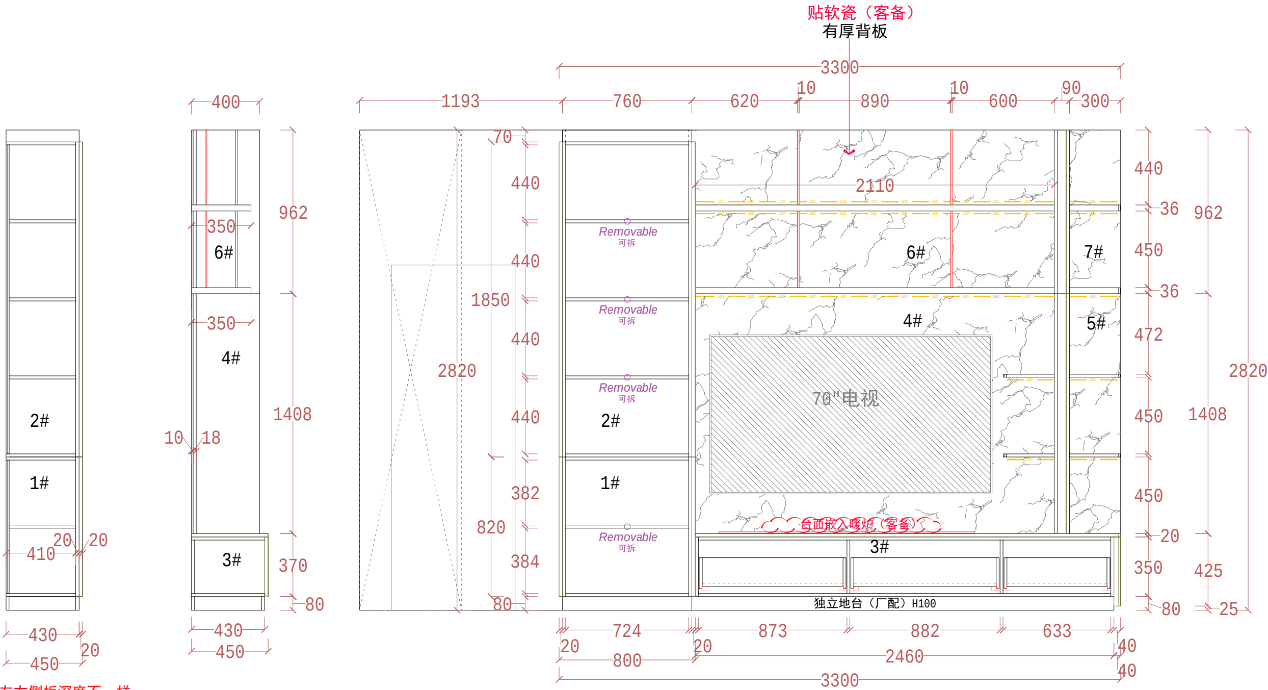
SECTION VIEW 1 SECTION VIEW 2
