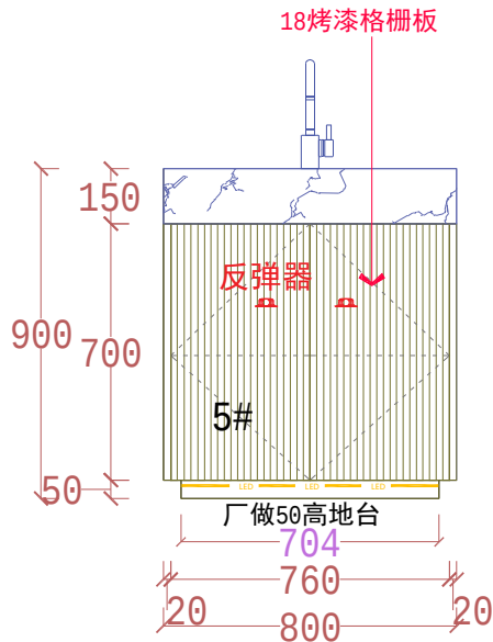
ELEVATION C
