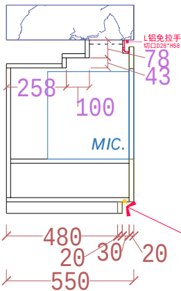
SECTION VIEW 1
