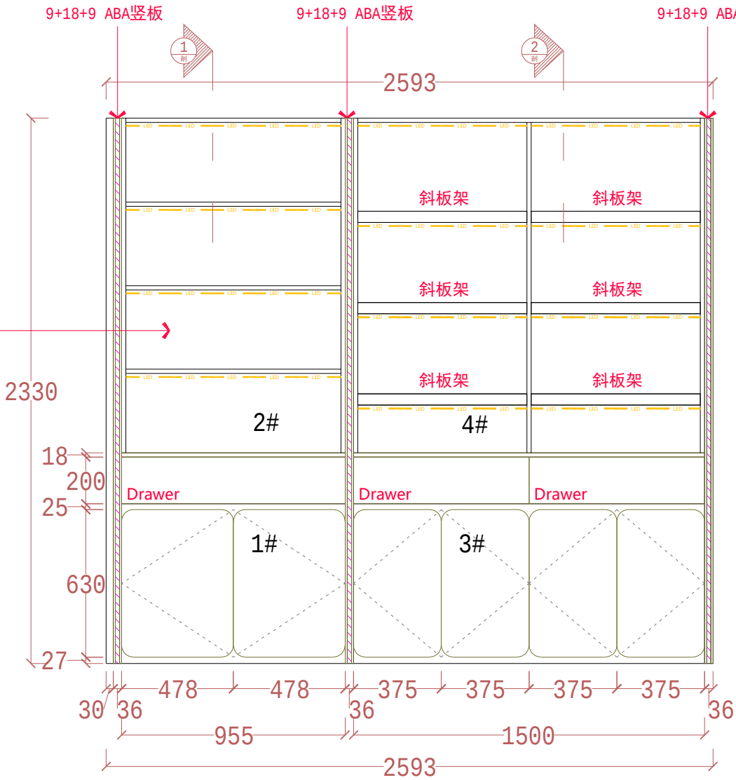
OUTSIDE VIEW
