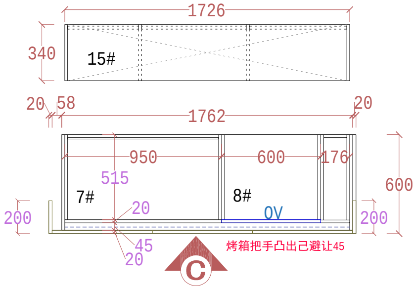
PLAN VIEW floor
