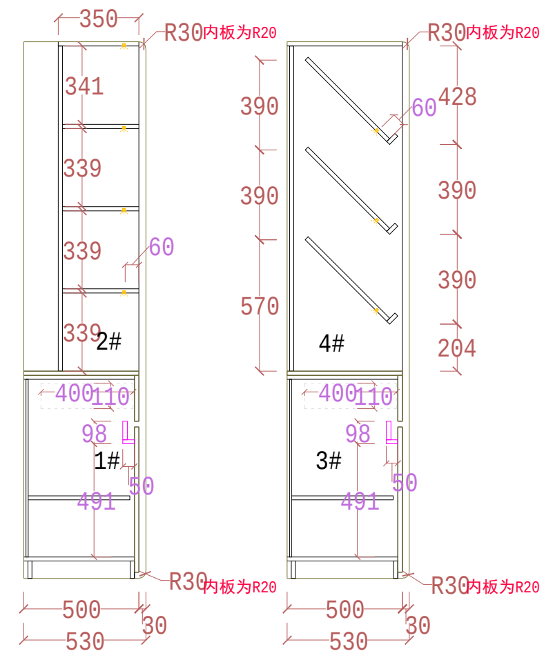
SECTION VIEW 1 SECTION VIEW 2
