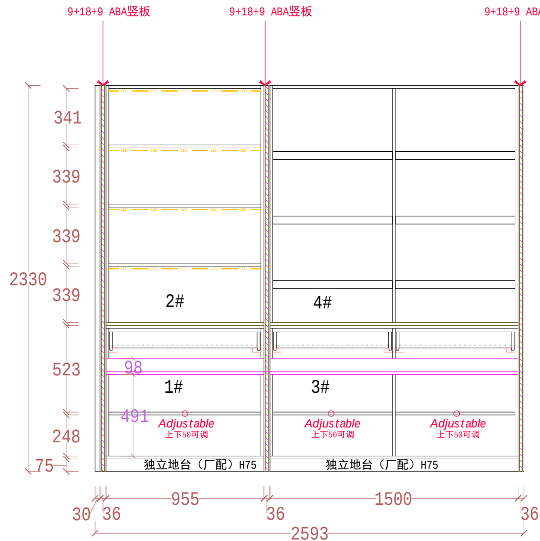
INNER VIEW
